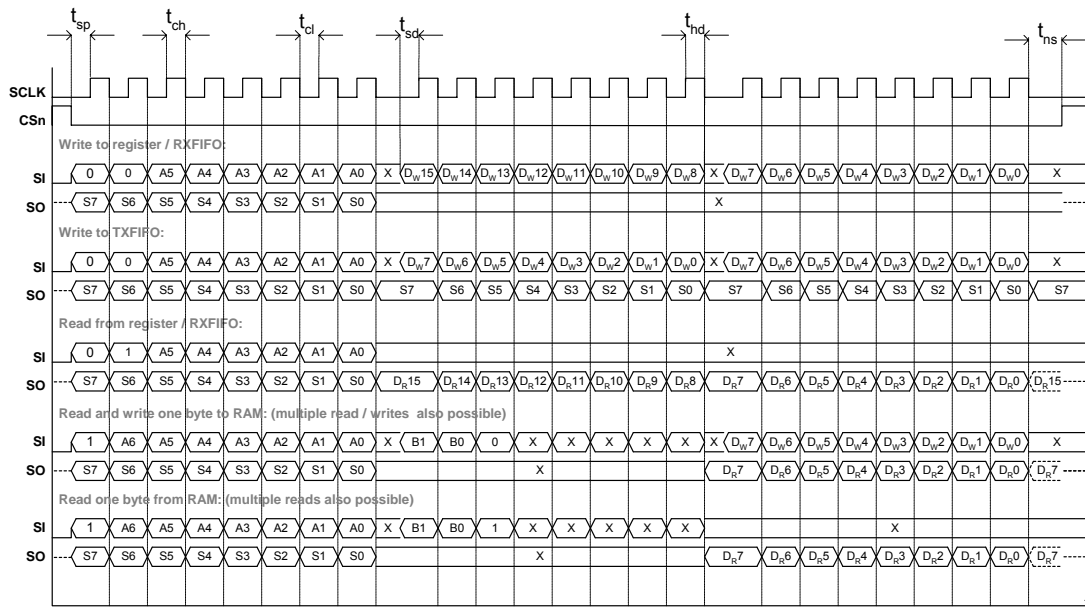
Figure 9. SPI timing diagram
