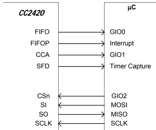
Figure 12. Microcontroller interface example
