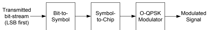
Figure 6. Modulation and spreading functions [1]
