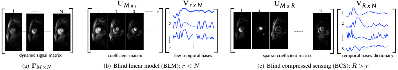
Fig. 1: Comparison of BCS and BLM representations of dynamic imaging data: The Casorati form of the dynamic signal \Gamma is shown in (a). The BLM and BCS decompositions of \Gamma are shown respectively in (b), (c). BCS uses a large over-complete dictionary, unlike the orthogonal dictionary with few basis functions in BLM. Note that the coefficients/ spatial weights in BCS are sparser than that of BLM. The temporal basis functions in the BCS dictionary are representative of specific regions, since they are not constrained to be orthogonal. For example, the 1st, 2nd columns of \mathbf{U}_{M \times R} in BCS correspond respectively to the temporal dynamics of the right and left ventricles in this myocardial perfusion data with motion. We observe that only 2-3 coefficients per pixel are sufficient to represent the dataset.
