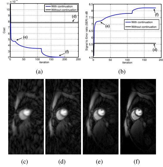
Fig. 2: (a): Cost in (3) v/s iteration, (b): SER (dB) v/s iteration, (c): Direct IFFT reconstruction for reference. A spatial frame of the reconstructions (d): without continuation, fixed \beta = 10^{10} , (e): with low \beta = 10^5 and (f): with continuation, start with \beta = 10^5 and increment till \beta = 10^{10} . The cost with continuation decreases monotonically avoiding any possible local minima as seen while fixing \beta to a large value in (d). Specifically (d) gets stuck in modeling the basis functions corresponding to error artifacts; (compare d and c). Also shown is the iterate during low \beta in (e), which is an equivalent nuclear norm solution. As \beta is increased during continuation, the algorithm converges to the BCS solution in (f).
