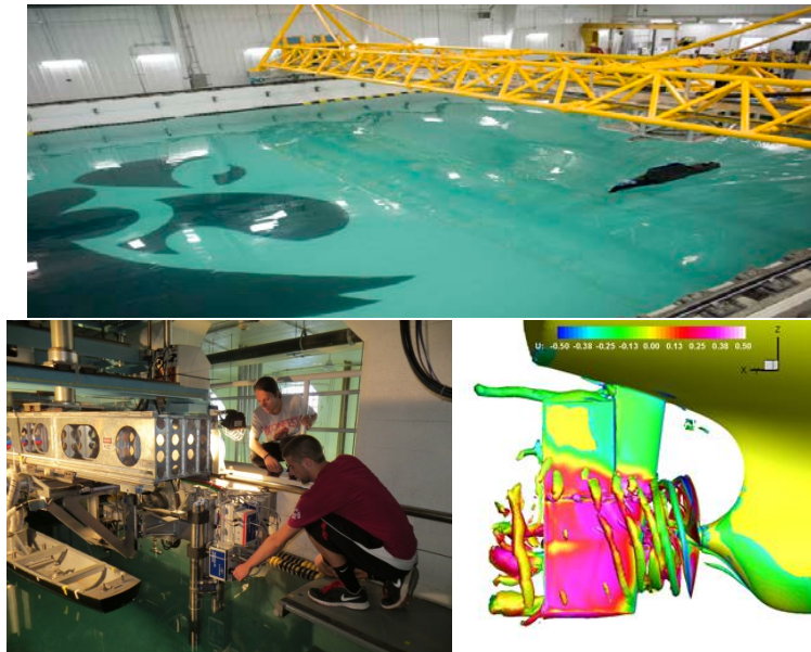
IIHR experimental wave basin (top), and towing tank (bottom left) facilities and computational CFDShip-Iowa code (bottom right)
