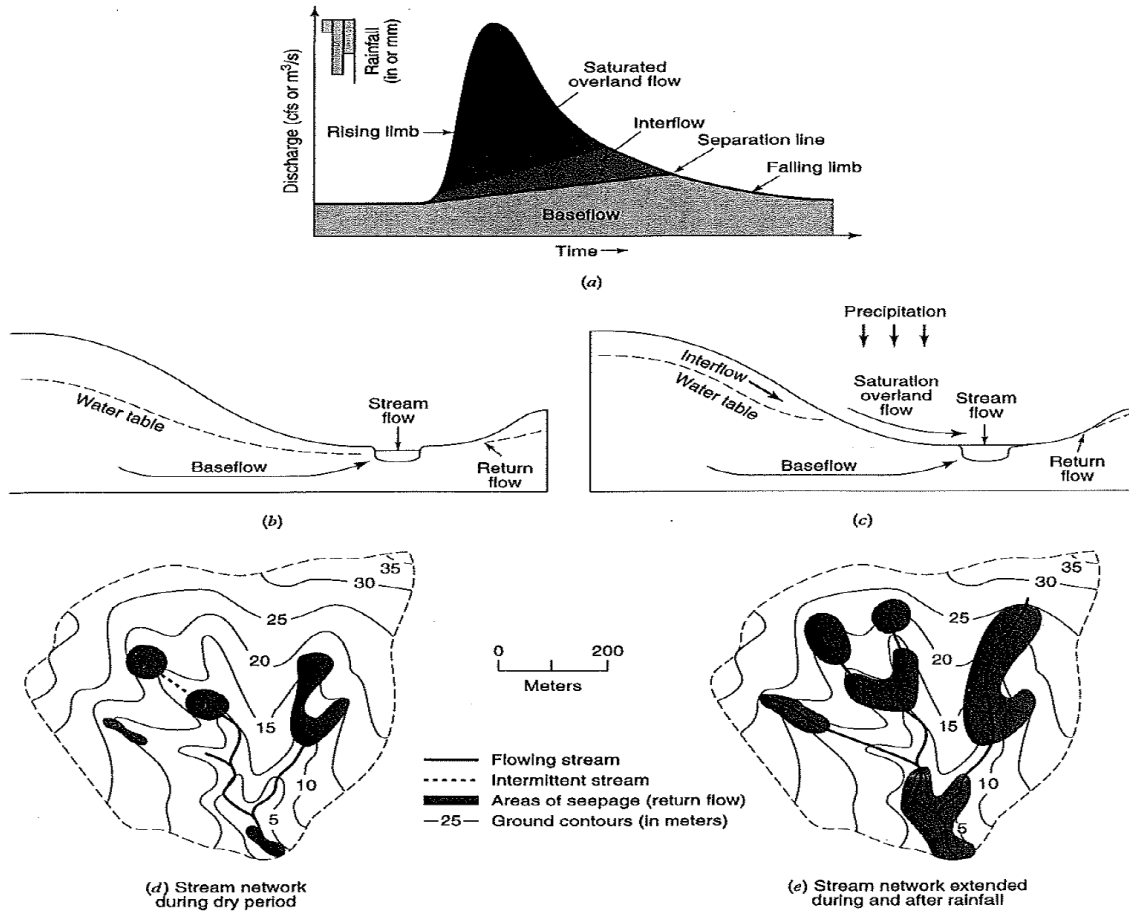
Figure 8.1.3 (a) Separation of sources of streamflow on an idealized hydrograph; (b) Sources of streamflow on a hillslope profile during a dry period, (c) During a rainfall event. (d) Stream network during dry period. (e) Stream network extended during and after rainfall (from Mosley and McKernan (1993)).
