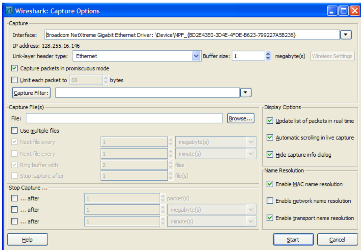
Figure 3: Wireshark Capture Options Window
