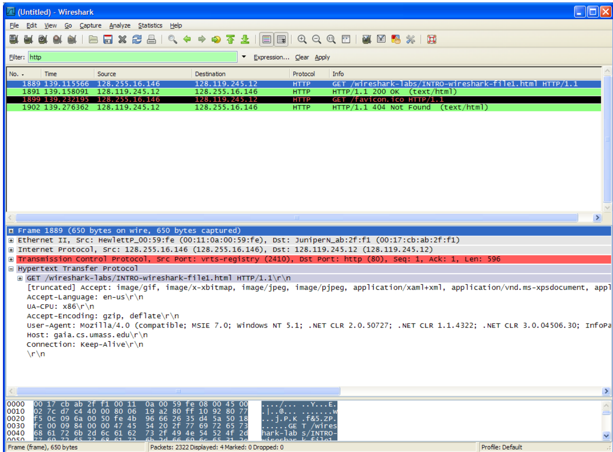
Figure 5: Wireshark display after step 9
