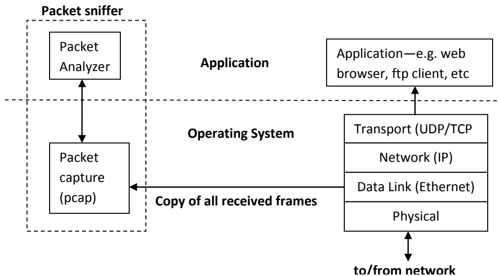
Figure 1: Packet sniffer structure
