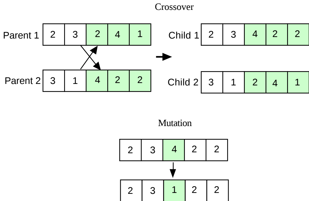
Figure 4. Crossover and Mutation for GAs.
