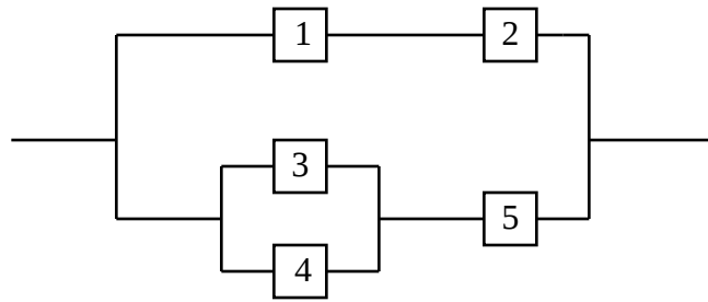
Figure 2. The series-parallel system.
