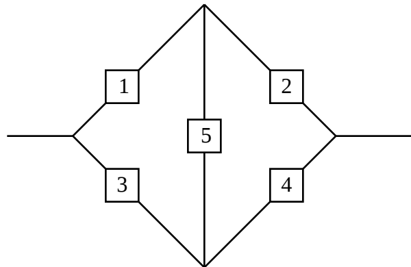
Figure 3. The complex (bridge) system.
