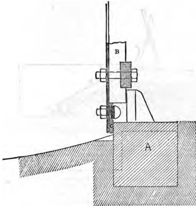
Fig. 278.—Arrangement of bottom of counter-wicket. A, sill; B, counter-wicket; C, India-rubber backing.
