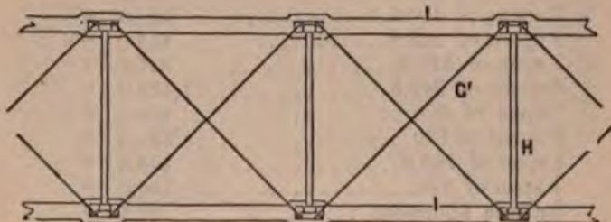
Fig. 180—Plan of the top of the bridge. I, top chord. H, cross-tie or strut. C', upper horizontal tie.
