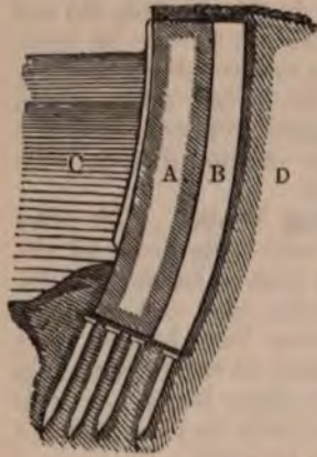
Fig. 69—Represents a section A of a wall with a curved face and back, and an elevation B of the counterforts. C, water. D, embankment behind the wall. a, fender beams of timber.
