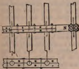
Fig. 147—Plan O, elevation M, and cross section N, showing the arrangement of the capping of the foundation piles with the uprights. a , piles. b , capping of four beams bolted together. c , uprights.
