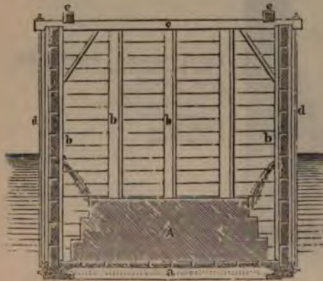
Fig. 54 represents a cross section and interior view of a caisson. The boards in this figure are represented as let into grooves in the vertical pieces, instead of being nailed to them on the exterior.
