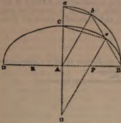
Fig. 115—Represents an oval curve of three centres, the arcs of which are each 60^\circ . DB, span of the curve, AC, rise, P, O, and R, centres of the arcs of 60^\circ . DCB is the intrados.
