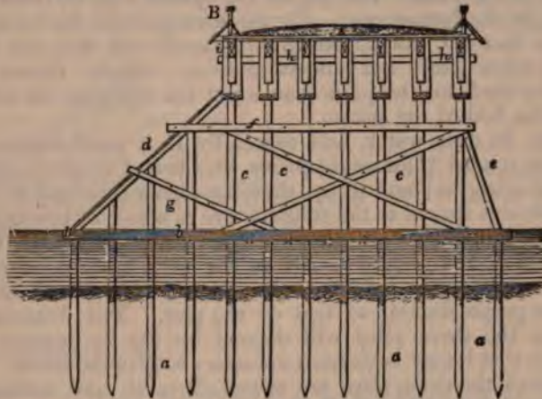
Fig. 146—Elevation of a wooden pier. a, a , piles of substructure. b, b , capping of piles arranged to receive the ends of the uprights c, c , which support the string-pieces f, f . d , upper fender beam. e , lower fender beam. f, f , horizontal ties bolted in pairs on the uprights. g, g , diagonal braces bolted in pairs on the uprights. h, h , capping of the uprights placed under the string pieces. A , roadway. B , parapet.
