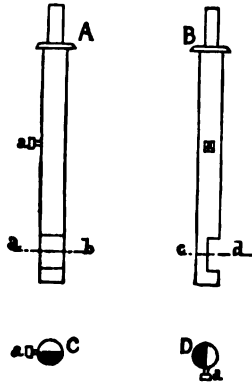
Fig. 260.—A, front elevation, and B, side elevation of jack-post, with escapement closed; C, section on a b ; D, section on c d . In all four a is the set screw.
