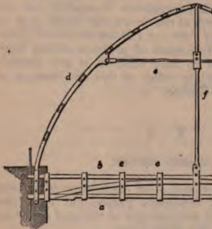
Fig. 166—Represents an open beam of wrought iron consisting of a top and bottom rail a and b , with an intermediate curved piece, the whole secured by the pieces c , c , in pairs bolted to them. d , e , and f represent the parts of a truss of a curved light roof, connected with the open beam; and also the manner in which the whole are secured to the wall.
