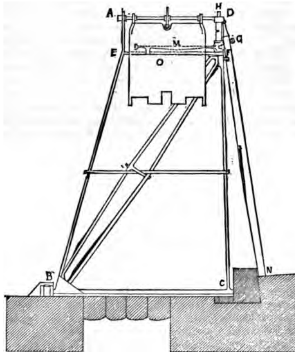
Fig. 256.—Side elevation of trestle on the Belgian Meuse. E B O F, trestle; B E, down-stream stile; O F, up-stream stile; E F, cap; B C, axle; M, movable bar resting against cap; O, attached floor; A D, axle of floor; H, square end of jack-post; G N, needle; G, eye on needle.
