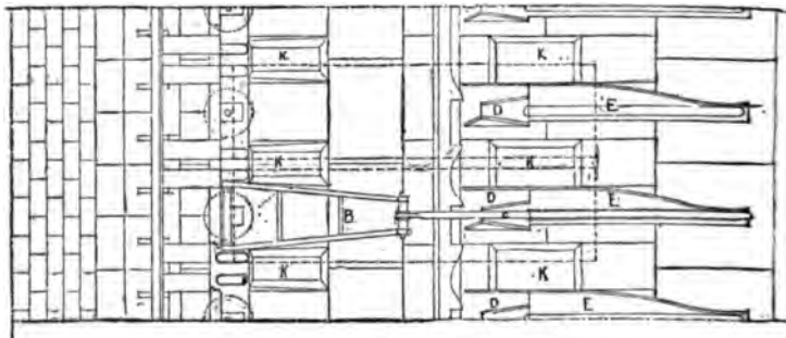
Fig. 263.—Plan of Chanoine dam. B, horse; C, prop; D, hurter; E, slide; F, sill; G, trip-bar; K K, pillows. Dotted rectangles show position of panels when down.
