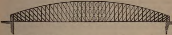
Fig. 187.—Kulenberg Bridge. Span between the abutments, 152 meters. Total length, including the parts on the abutments, 156.8 meters (about 515 feet). Length of each bay, 4 meters. Depth of the truss at the centre, 29 meters.
