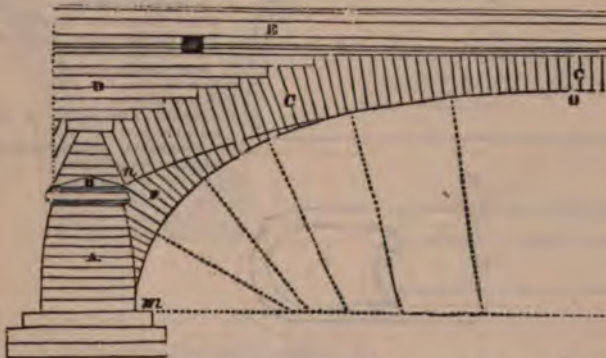
Fig. 133—Represents in elevation the combinations of the same elements as in Fig. 132, from the bridge of Neuilly, and oval of eleven centres. om , curve of intrados. on , arc of circle traced on the head of the bridge.
