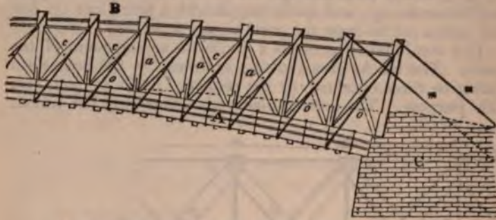
Fig. 155—Represents a side view of a portion of the open-curved rib of the bridge over the Schuylkill at Philadelphia.
