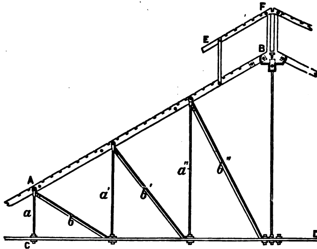
Fig. 213.—Ordinary roof of a gas-house. A, B, is the main rafter. a, a'' are vertical tie-rods. b, b'' are braces. C, D, is the main tie. E, F, is the ventiator.
