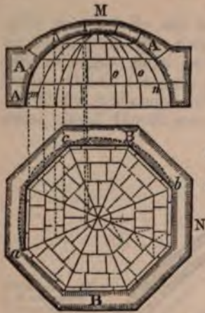
Fig. 77—Represents a section M of the voussoirs and an elevation of the soffit, with a plan N of the soffit of an octagonal-cloistered dome. The letters refer to the same parts as in Fig. 75.
