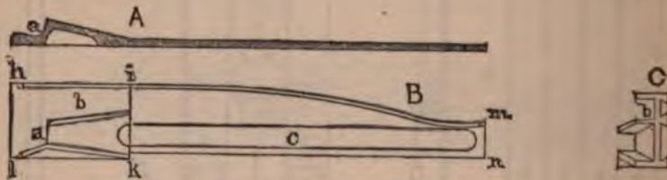
Fig. 265.—A, longitudinal section; B, plan; C, end view of hurter and slide; h i k l , hurter; m n k , slide; a , prop seat; b , passage; c , groove.
