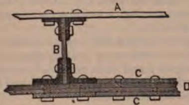
Fig. 190—Victoria Bridge. Web plates and top plates at centre of tube. A, the bar 6" x 9".75 B, web plate. C C, cover plates. D, top plates. E, bottom plates. F, heavy wooden beams on which rail H rests. G, cross timber to connect beams F.
