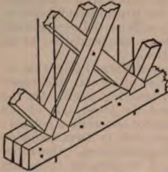
Fig. 86 is a perspective view of a part of one panel of the Howe truss, and shows quite clearly how the parts are arranged. For an analysis of these structures, see Wood's Treatise on Bridges and Roofs.
