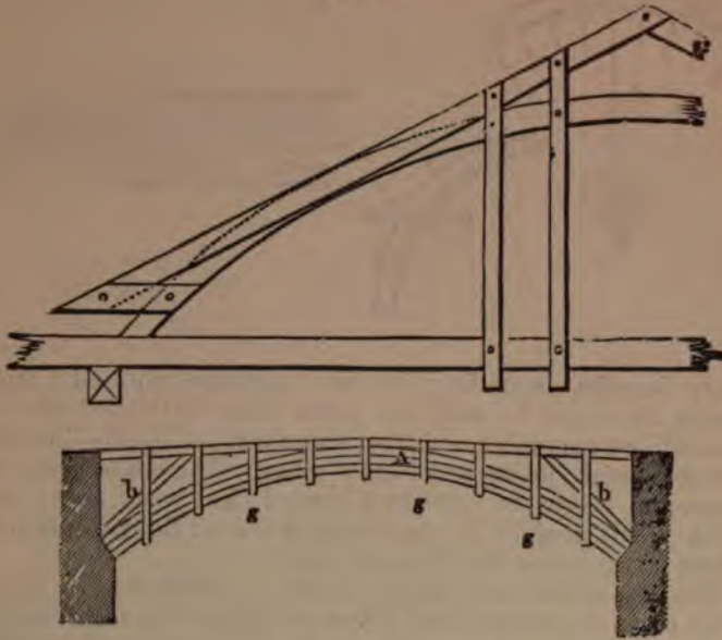
Fig. 112—Represents a wooden arch A formed of a solid built beam of three courses which support the beams c, c by the posts g, g which are formed of pieces in pairs. b, b, inclined struts to strengthen the arch by relieving it of a part of the load on the beams c, c.
