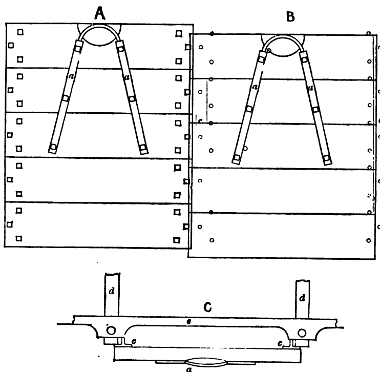
Fig. 272.—A, front view; B, back view; C, plan of Boulé gates; a, a, handle; c, c, T-iron guides; d, d, cap of trestle; e, connecting bar.
