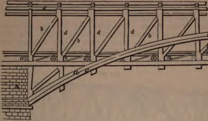
Fig. 156—Represents a side view of a portion of a rib of Barr's bridge. a, a , arch timbers. d, d , queen-posts. b, b , braces. c, c , chords.
