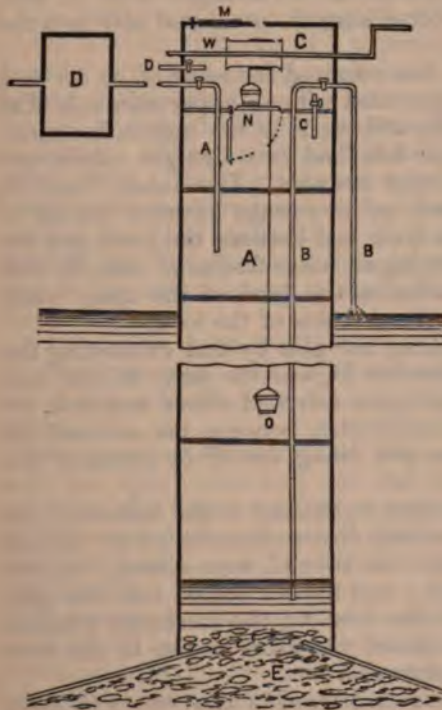
Fig. 55.—Longitudinal section of a pneumatic pile A, air-lock C, and exhaust vessel D. A, exhaust tube between A and D. B, water discharge-tube. C, equilibrium tube between the lock and chamber of the pile. D, equilibrium tube between lock and exterior air. M, upper man-hole and valves. N, lower man-hole and valves. W, windlass and gearing. E, concrete underpinning as practised at Harlem bridge.
