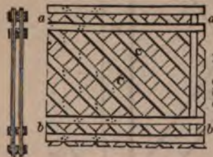
Fig 153.—Represents an elevation A, and end view, B, of a portion of Town's truss. a, a, top strings. b, b, bottom strings. c, c, diagonal braces.
