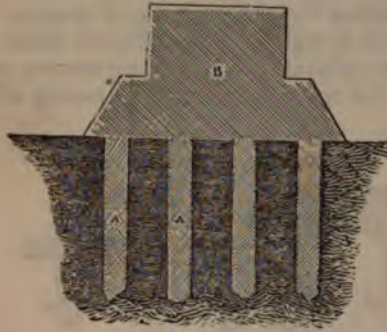
Fig. 42.—Represents a section of a foundation bed made by filling holes with sand. A, holes filled with sand. B, masonry.
