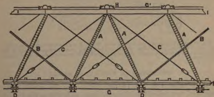
Fig. 178.—Side view of panels of a Post Truss. A A are struts. B B, main ties. C C, counter ties. E E, bottom chords. I I, top chords. D, ends of floor-beams. G, lower horizontal diagonal ties. G', upper horizontal diagonal ties.
