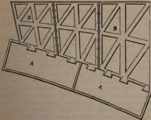
Fig. 163—Represents a portion of a cast-iron plate arch with an open cast-iron beam. A, A, segments of the arch. B, B, panels of the open beam connected at the joints a b .
