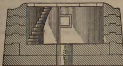
Fig. 26.—Vertical section and interior elevation above foundation courses.
