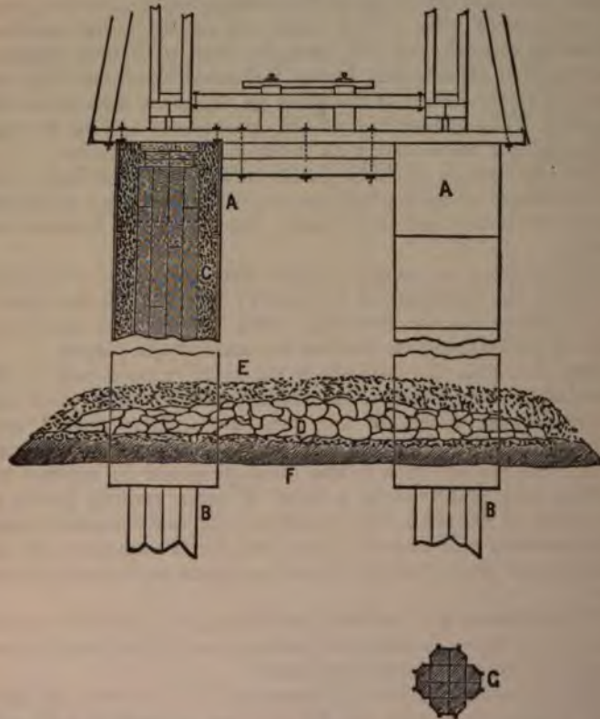
Fig. 30 represents a section and elevation of a pier of the Seekonk river bridge. A, outside cover of metal. B, clusters of wooden piles. C, inside filling of concrete. D, loose stone. E, slag. F, crust of shells. G, cross section of wooden clusters.
