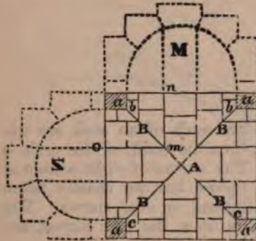
Fig. 74—Represents the plan of the soffit and the right sections M and N of the cylinders forming a groined arch. aa , pillars supporting the arch. bc , groins of the soffit. om, mn , edges of coursing joints. A , key-stone of the two arches formed of one block. B, B , groin stones of one block below the key-stone forming a part of each arch.
