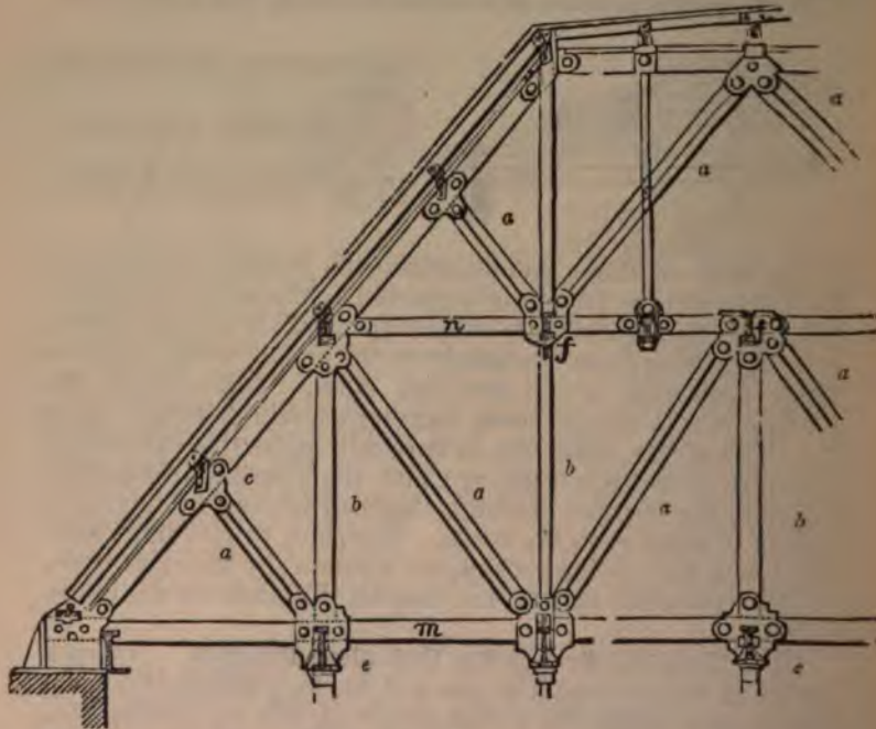
Fig. 210—Represents the half of a truss for the same building composed of wrought and cast iron. a, a , feathered struts of cast-iron. b, b , suspension bars in pairs. m, n , tie and straining bars. e, e , and f, f , cross sections of beams resting in the cast-iron sockets connected with the suspension bars.
