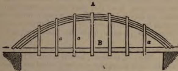
Fig. 113—Represents a wooden arch of a solid built beam A which supports the horizontal beam B by means of the posts a, a. The arch is let into the beam B, which acts as a tie to confine its extremities.
