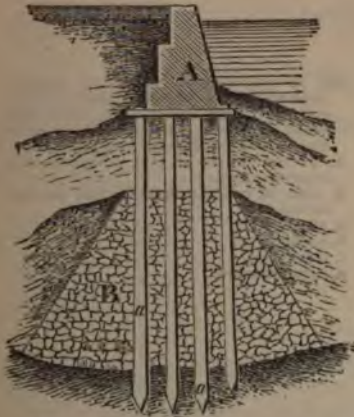
Fig. 43.—Represents the manner of using loose stone to sustain piles and prevent them from yielding laterally. A, section of the masonry. B, loose stone thrown around the piles, a.
