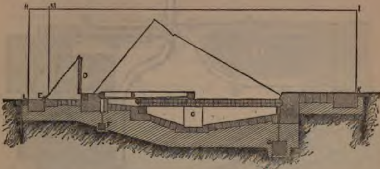
Fig. 274.—Section of bear-trap gate down. A, lower gate; B, upper gate; C, entrance for water from passage in pier; D, auxiliary gate; E, trigger; E M, trigger rod; F and G, anchorages; H I K L, pier.
