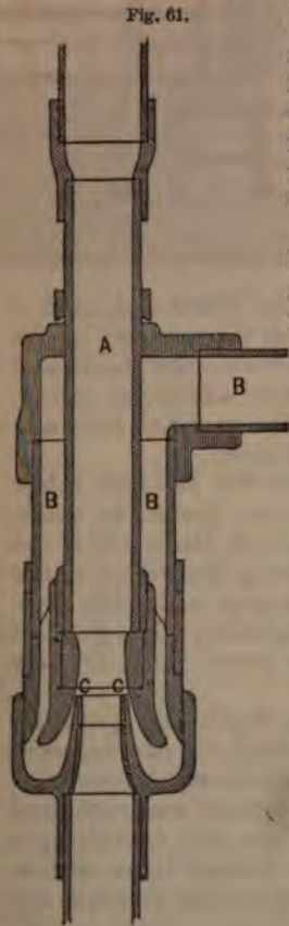
Fig. 61, represents a vertical section of a sand-pump. A, pump barrel. B, injection pipe. C, annular jet.
