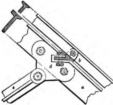
Fig. 212—Represents the arrangements of the parts at the joint c in Fig. 210. A, side view of the pieces and joint. a, principal rafter of the cross section B. b, common rafter of the cross section C. c, cross section of purlins and joint for fastening the common rafters to the purlins. d, cast-iron socket arranged to confine the pieces a, b, c, e.
