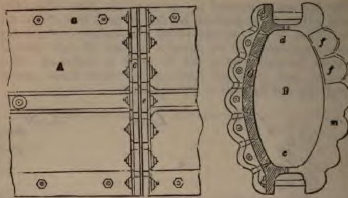
Fig. 165.—Represents a side view A, and a cross section and end view B, through a joint of M. Polonceau's tubular arch. a , a , top flanch, b , b , bottom flanch of the semi-segments united along the vertical joint c through the axis of the rib. g A , side view of the joint between the flanches e , e of two semi-segments. m , inner side of the flanches. c , cross section of a semi-segment and top and bottom flanches. f , f , thin wedges of wrought iron placed between the end flanches of the semi-segments to bring the parts to their proper bearing.
