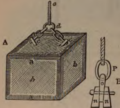
Fig. 27.—Represents a perspective view, A, of a block of stone with draughts around the edges of its faces, and the intermediate space axed, or knotted, and its tackling for hoisting; also the common iron lewis, B, with its tackling. a , draughts around edge of block. b , knotted part between draughts. c , iron bolts with eyes let into oblique holes cut in the block. d and e , chain and rope tackling. n, n , side pieces of the lewis. o , centre piece of lewis with eye fastened to n n by a bolt. p , iron ring for attaching tackling.
