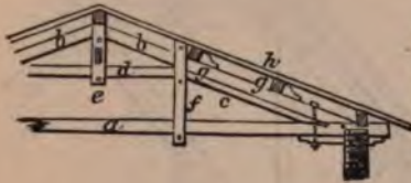
Fig. 209—Represents a roof truss for wide spans. a , tie-beam. b , b' , principal rafters, c , short rafters abutting against the straining beam d . e and f , king and queen posts in pairs. g , g' , pairs supporting common rafters h .
