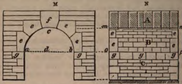
Fig. 73.—Represents an elevation M of the head of a right cylindrical arch, and a section N through the crown of the arch A, with an elevation B of the soffit and the face C of the abutment.
