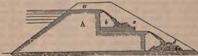
Fig. 242—Represents a section of a waste-weir divided into two falls. A, body of the dam. a, top of the waste-weir. b, pool, formed by a stop-plank dam at c, to break the fall of the water. d, covering of loose stone to break the fall of the water from the pool above.
