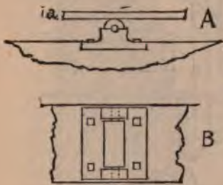
Fig. 207.—A, side view, and B, plan of roller and sill; a, trip-bar resting on roller.
