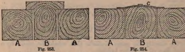
Fig. 253.—T-needle B covering intervals between it and ordinary needles, A A. Fig. 254.—Needle B, with india-rubber facing, C, covering intervals between B and A A.
