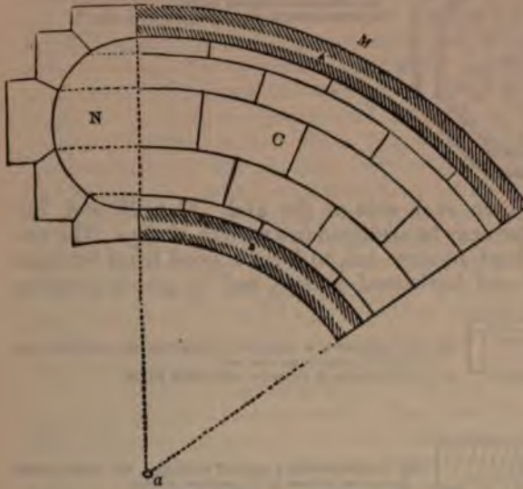
Fig. 76.—Represents a plan M of the abutments A and B, and the soffit C of an annular arch. N, right section of the arch. a, position of vertical axis around which the section N is revolved.
