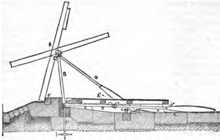
Fig. 262.—Section of Chanoine dam, showing wicket down, up, and swung. A, panel; B, horse; C, prop; D, hurter; E, slide; F, sill; G, trip-bar; H, anchoring bolt; I, anchoring disc; K K, pillows; O, axis of oscillation. A', B', C' show panel, horse, and prop when down. Dotted lines show panel swung.
