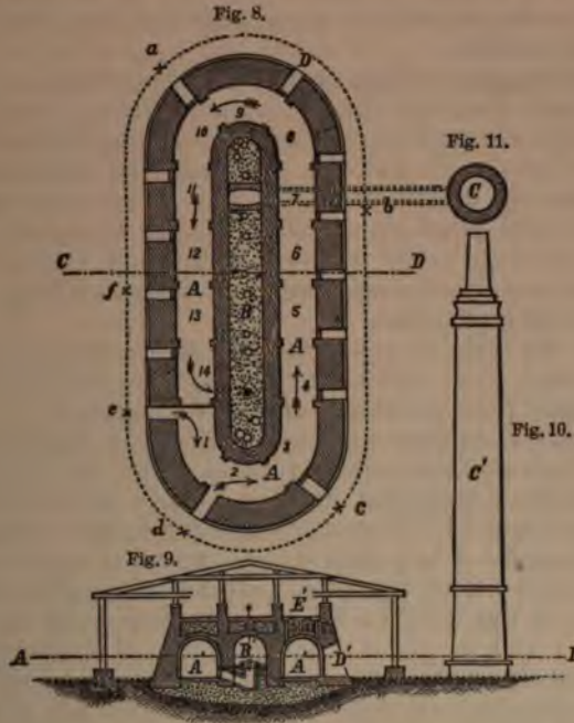
Fig. 8. Horizontal section of kiln on A B, Fig. 9. Fig. 9. Vertical section on C D, Fig. 8. Fig. 10. Elevation of chimney. Fig. 11. Section of chimney at A B, Fig. 10. A, A', Burning chamber. B, B', Smoke chamber. C, C, Chimney. D, Doorways. a, b, Lime-stone in process of burning. b, c, do. do. of cooling. c, d, do. do. of drawing. d, e, do. do. of setting up. e, f, do. do. of drying. f a, do. do. of taking up waste heat.
