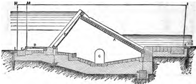
Fig. 273.—Section of bear-trap gate raised. A, lower gate; B, upper gate; C, entrance for water from passage in pier; D, auxiliary gate; E, trigger; E M, trigger rod; F, G, anchorages; H I K L, pier.
