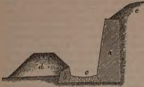
Fig. 45 represents the manner of buttressing a sustaining wall in front by the action of a counter-pressure of earth transmitted to the wall by a reversed arch. a , section of sustaining wall. b , section of sustaining wall of embankment, d . c , section of reversed arch. d , section of embankment from which counter-pressure comes. e , section of embankment behind sustaining wall.
