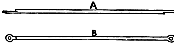
Fig. 253.—A, elevation: B, plan of down-stream connecting bar. The holes at the ends of the bar fit on pins, B, Fig. 248.
