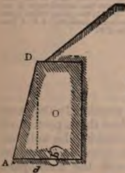
Fig. 66—Represents a section O of a retaining wall with a sloping face AD. P, section of the embankment.
