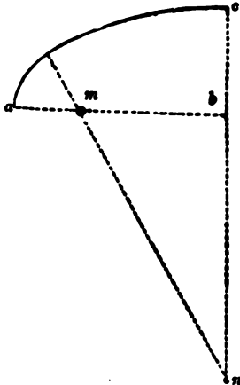
Fig. 117—Represents the half of an obtuse or surbased curve of four centres, ab , half span, bc , rise, m and n , centres of the half curve ac .
