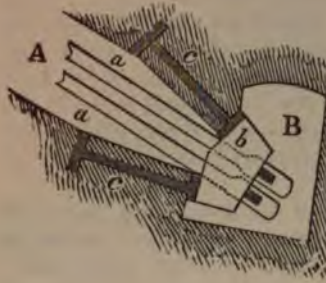
Fig. 193—Shows the manner in which the side main-chains are anchored.
