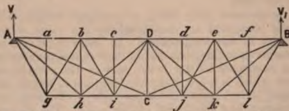
Fig. 177—Fink Truss. A B the upper chord, g l the lower chord, \alpha \rho, b h , etc., are posts. A C, C B long suspension-rods. A h, h D, etc., secondary suspension-rods.
