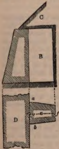
Fig. 70.—Represents a section A and plan D of a wall, and an elevation B, and plan E of a trapezoidal counterfort.
