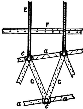
Fig. 185—Shows a side view of a portion of the arch. G G are diagonal posts which are trussed, as shown in Fig. 183, for connecting the two arches together. The other letters refer to the same parts as in Figs. 183 and 184.
