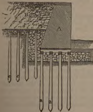
Fig. 46 represents the manner of relieving a sustaining wall from the lateral action caused by the pressure of an embankment on the subsoil by means of a platform built behind the wall. A , section of the wall. B , section of embankment. a , piles supporting the grillage and platform of A . b , loose stone, forming a firm bed under the platform. c , piles supporting the platform d behind the wall.
