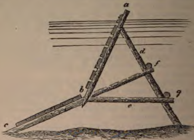
Fig. 247—Represents a section of the timber wing-dams on the Po, formed of plank nailed on the inclined pieces of the ribs. a b and b c , inclined faces of the dam, the first making an angle of 63^\circ , and the second of 23^\circ with the horizon. d and e pieces of the rib. f and g horizontal pieces connecting the ribs.
