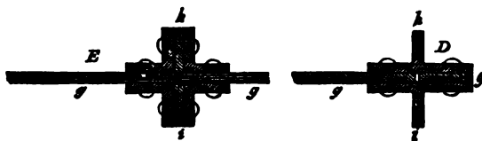
Fig. 169—Represents a horizontal cross-section of the T irons and side plates. D , cross-section near centre of bridge. E , cross-section near the piers. g , plates of the sides. A , exterior T irons. a , interior T irons.
