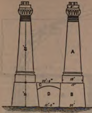
Fig. 198—End elevation of piers and connecting arch of bridge. A, shaft of the pier. B, pedestal. C, connecting arch. D, arched way for common road.
