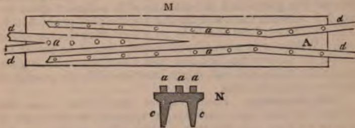
Fig. 232—Represents a plain M, and section N, of a fixed crossing plate. The plate A is of cast-iron, with vertical ribs c, c, on the bottom, to give it the requisite strength. Wrought-iron bars a, a, placed in the lines of the two intersecting rails d, d, are firmly screwed to the plate; a sufficient space being left between them and the rails for the flanch of the wheel to pass.
