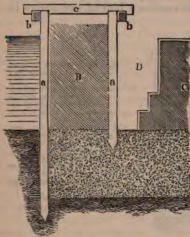
Fig. 53 represents a section of General Treussart's dam. A, bed of béton. B, puddling of dam. C, masonry of structure. a, square piles. b, wale pieces. c, cross piece.
