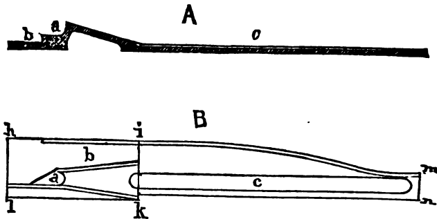
Fig. 260.—A, longitudinal section; B, plan of Pasquean's double-seated hurter and slide; a, prop seat; b, passage; c, groove; A i k l, hurter; i m n k, slide.
