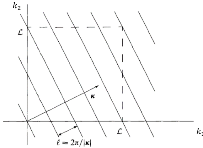
Fig. 6.8. A sketch of the Fourier mode corresponding to \underline{\kappa} = \kappa_0(4, 2, 0) . The oblique lines show the crests, where \Re(e^{i\underline{\kappa} \cdot \underline{x}}) = \cos \underline{\kappa} \cdot \underline{x} is unity.
