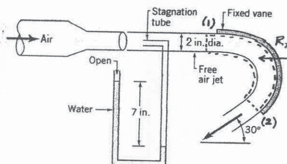
■ FIGURE P5.66
