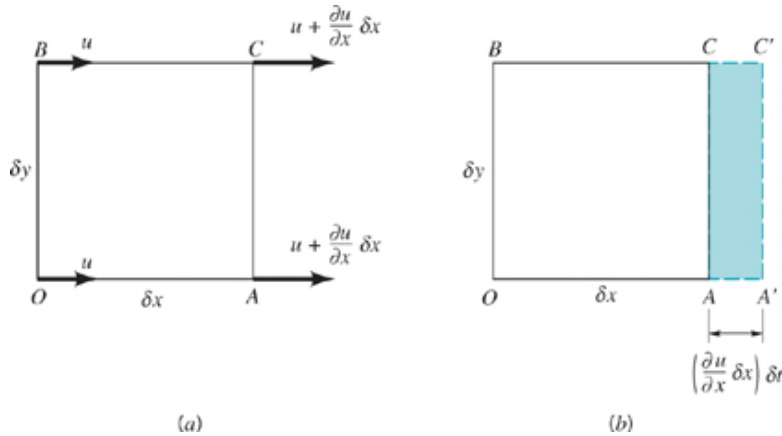
Linear deformation of a fluid element
