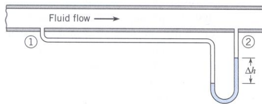
Differential manometer
