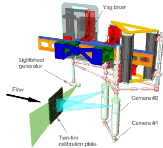
3D Stereo PIV System
