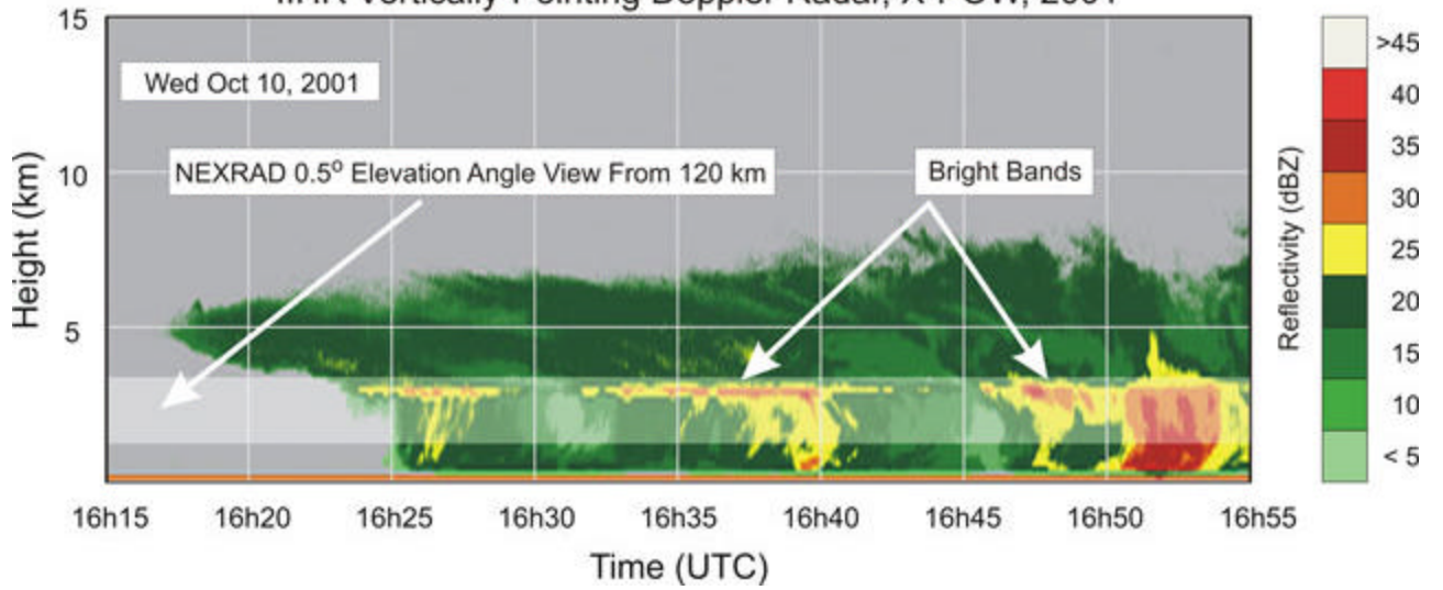
IIHR Vertically-Pointing Doppler Radar, X-POW, 2001
