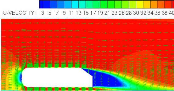
Figure 5: Flow field in the symmetry section colored by the stream-wise u-velocity predicted by the k-\varepsilon-v^2 model
