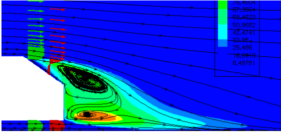
Figure 4: unsteady wake behind the body predicted using the k-\varepsilon-v^2 model
